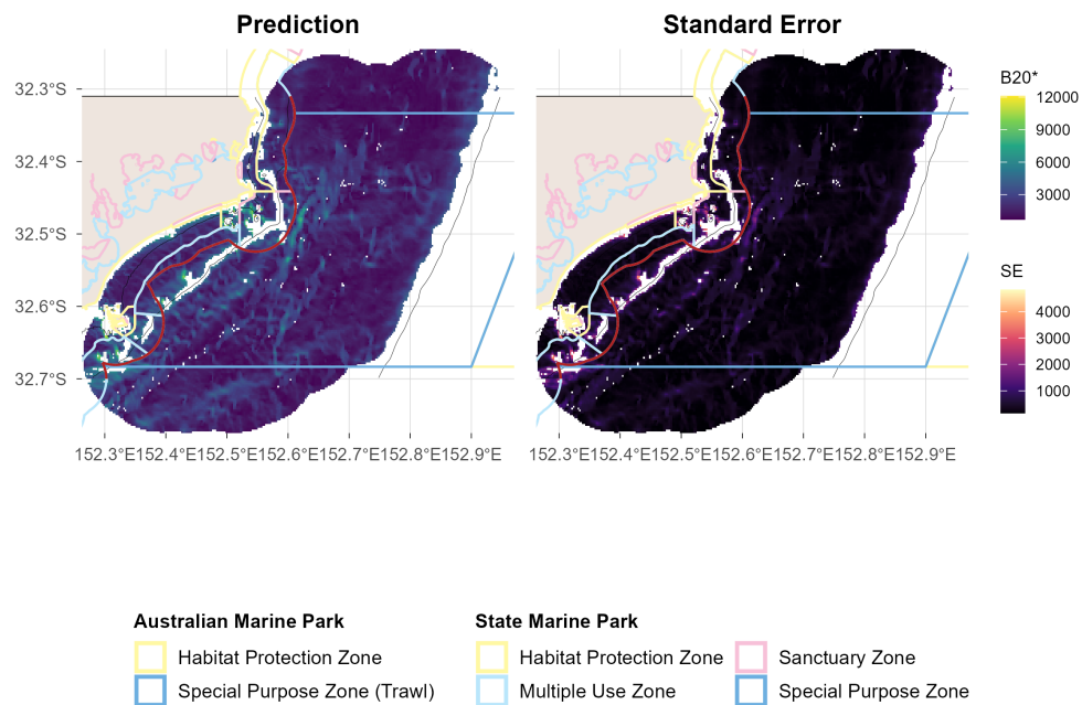
Figure A.9.3: Demersal fish - Large Reef Fish Index*: spatial plots of distribution probability and uncertainty from stereo-BRUV groundtruthing. Commonwealth and State marine park boundaries are shown. The red line delimits state and commonwealth waters. Bathymetric contours at 30, 70 and 200 m are shown.
