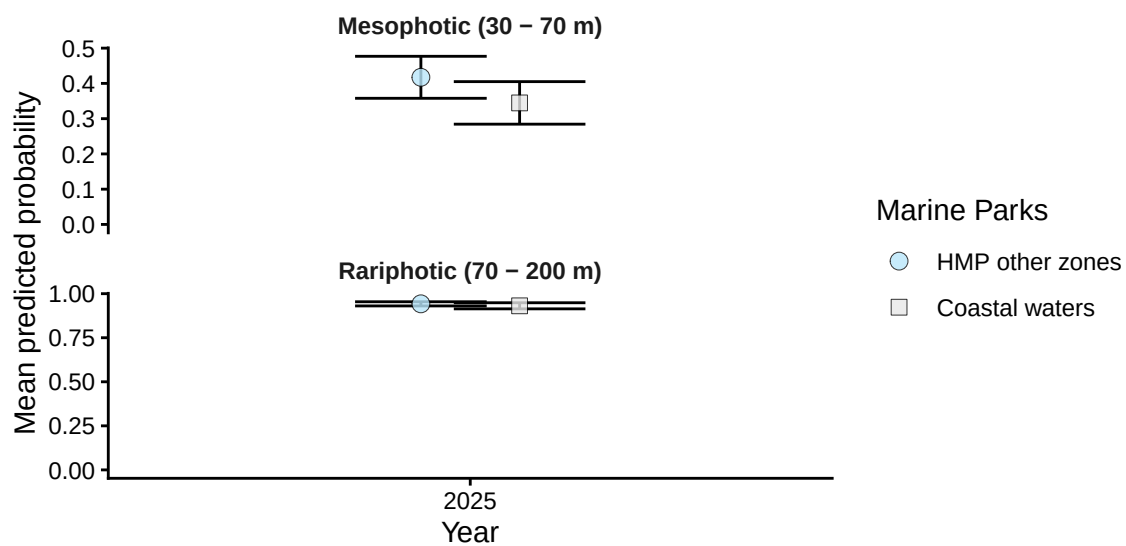
Figure A.4.1: Sediment: temporal plots by depth contour from stereo-BRUV groundtruthing. HMP = Hunter Marine Park (Commonwealth).
