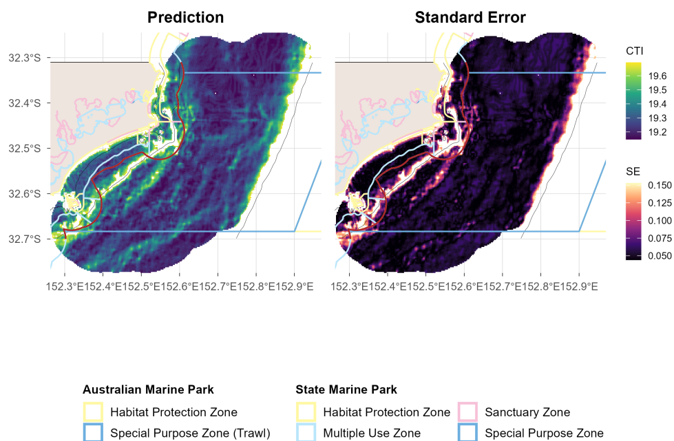
Figure A.10.3: Demersal fish - Reef Fish Thermal Index: spatial plots of distribution probability and uncertainty from stereo-BRUV groundtruthing. Commonwealth and State marine park boundaries are shown. The red line delimits state and commonwealth waters. Bathymetric contours at 30, 70 and 200 m are shown.
