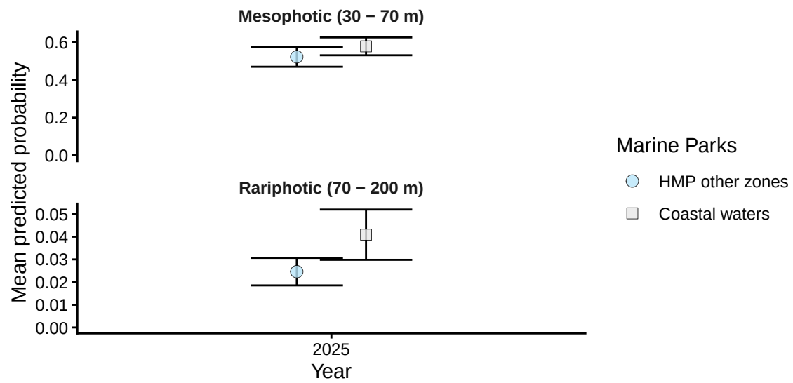
Figure A.5.1: Sessile invertebrates: temporal plots by depth contour from stereo-BRUV groundtruthing. HMP = Hunter Marine Park (Commonwealth).
