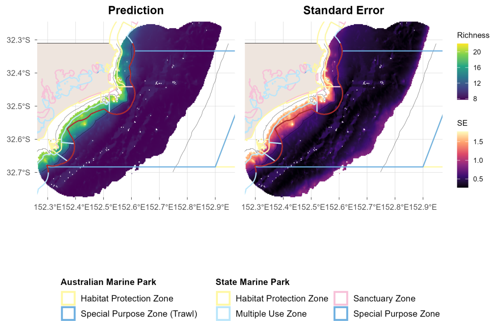
Figure A.7.3: Demersal fish - Species richness: spatial plots of distribution probability and uncertainty from stereo-BRUV groundtruthing. Commonwealth and State marine park boundaries are shown. The red line delimits state and commonwealth waters. Bathymetric contours at 30, 70 and 200 m are shown.
