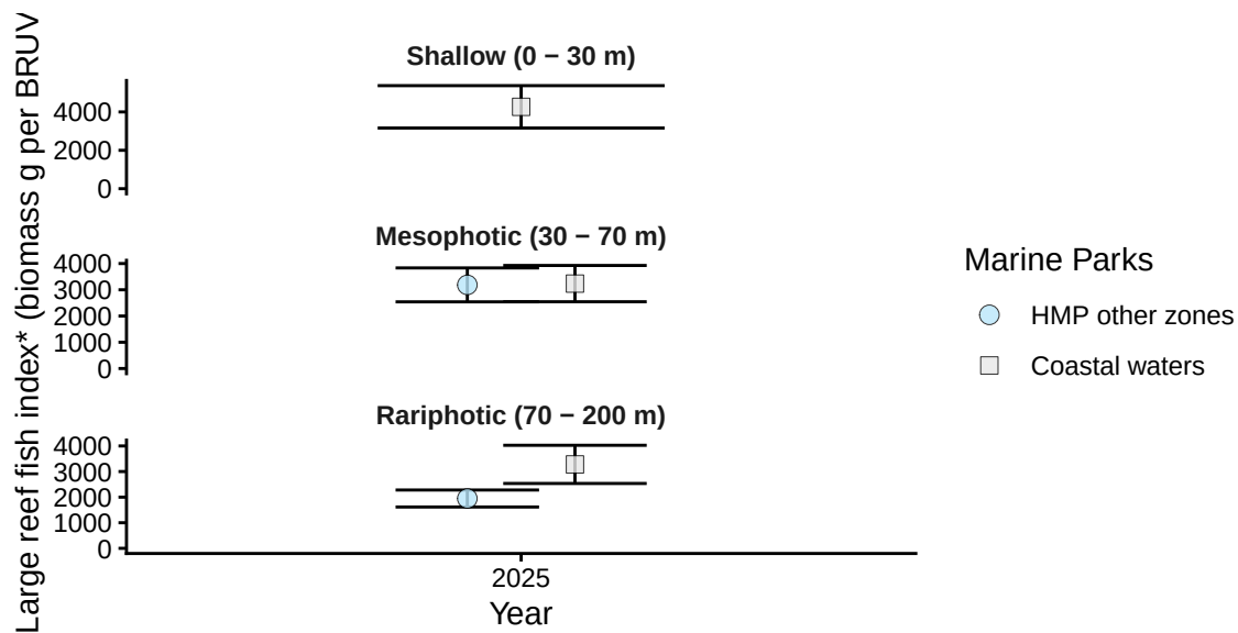
Figure A.9.1: Demersal fish - Large Reef Fish Index*: benchmark plots by zone and depth contour from stereo-BRUV groundtruthing. HMP = Hunter Marine Park (Commonwealth), PSGLMP = Port Stephens Great Lakes Marine Park (State). *Large Reef Fish Index representing the biomass of all fish greater than 20 cm (B20) has been adapted here for stereo-BRUV data by removing sharks and rays.
