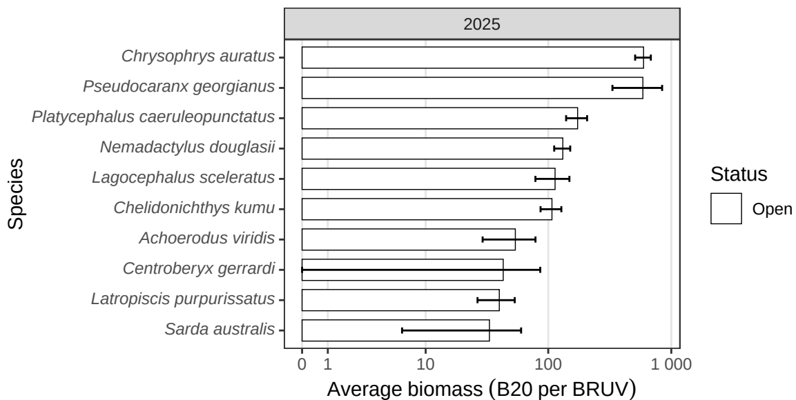
Figure A.9.2: Demersal fish - Large Reef Fish Index*: top 10 greatest biomass species (pooled across deployments) from stereo-BRUV groundtruthing in Hunter Marine Park (Commonwealth).
