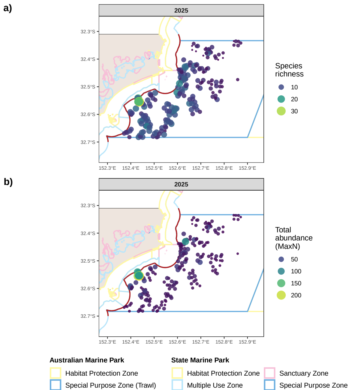
Figure A.6: Spatial distribution of observed species richness and total abundance (MaxN) per stereo-BRUV drop, pooled across all deployments. Commonwealth and State marine park boundaries are shown. The red line delimits state and commonwealth waters.
