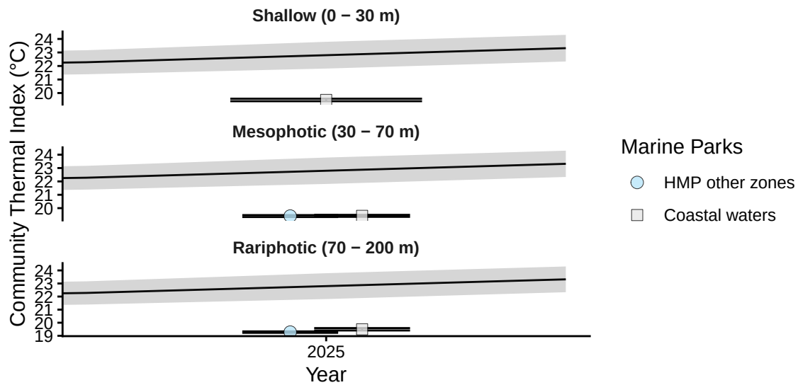
Figure A.10.1: Demersal fish - Reef Fish Thermal Index: benchmark plots by zone and depth contour, with monthly sea surface temperature (black line, grey band = SD) overlaid, from stereo-BRUV groundtruthing in Hunter Marine Park (Commonwealth).
