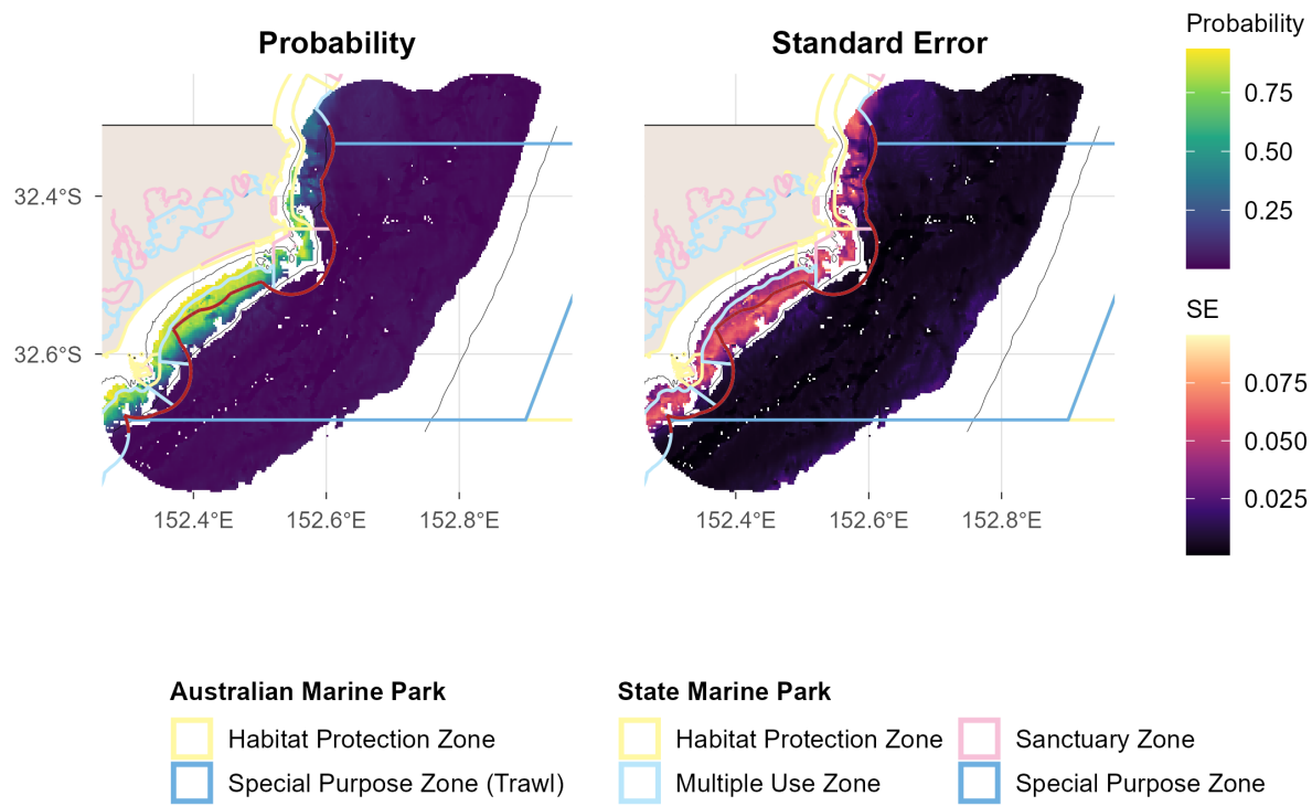
Figure A.5.2: Sessile invertebrates: spatial plots of distribution probability and uncertainty from stereo-BRUV groundtruthing. Commonwealth and State marine park boundaries are shown. The red line delimits state and commonwealth waters. Bathymetric contours at 30, 70 and 200 m are shown.
