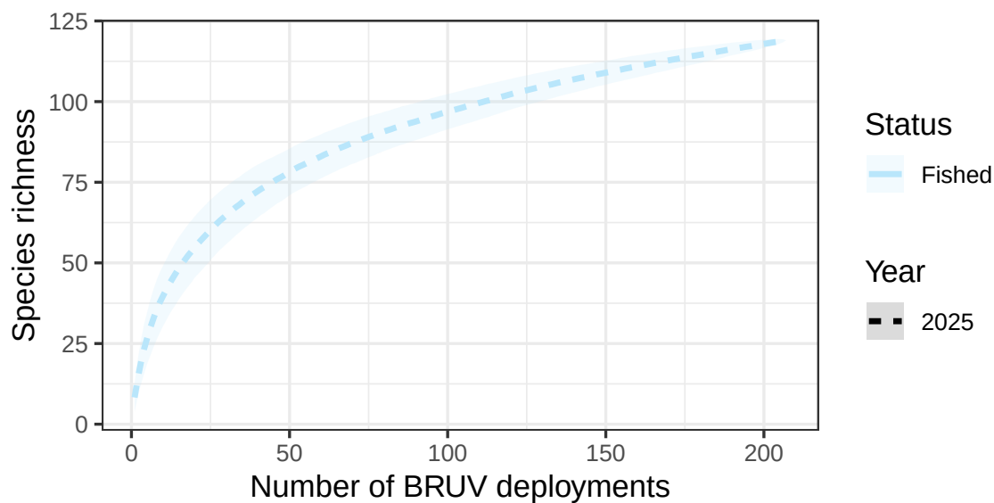
Figure A.7.2: Demersal fish - Species richness: species accumulation curve by year from stereo-BRUV groundtruthing in Hunter Marine Park (Commonwealth).
