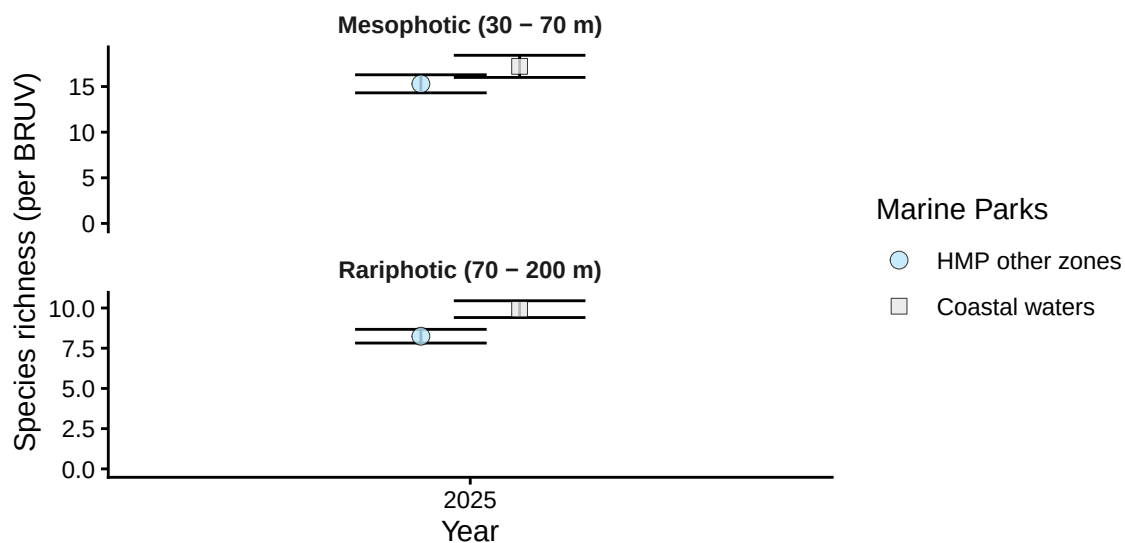
Figure A.7.1: Demersal fish - Species richness: benchmark plots by zone and depth contour from stereo-BRUV groundtruthing. HMP = Hunter Marine Park (Commonwealth).
