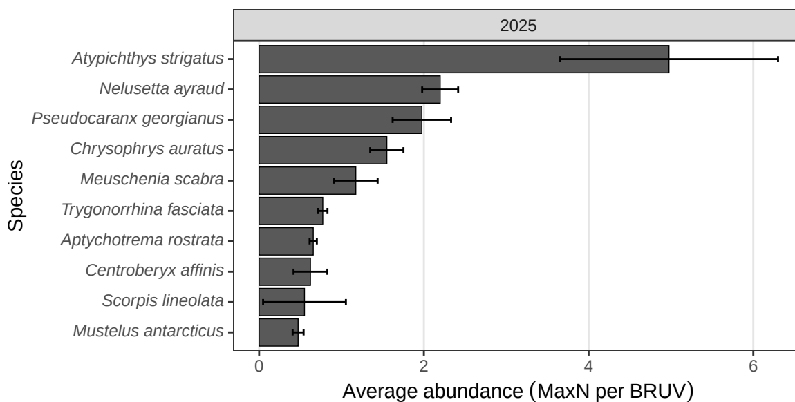
Figure A.8.2: Demersal fish - Total abundance: top 10 most abundant species (pooled across deployments) from stereo-BRUV groundtruthing in Hunter Marine Park (Commonwealth).
