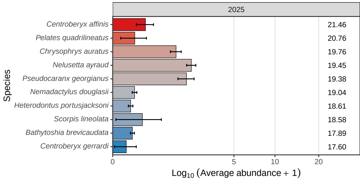
Figure A.10.2: Demersal fish - Reef Fish Thermal Index: species thermal niche of top 10 most abundant species (pooled across deployments) from stereo-BRUV groundtruthing in Hunter Marine Park (Commonwealth).
