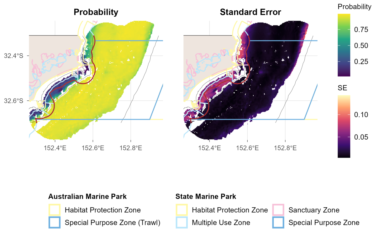
Figure A.4.2: Sediment: spatial plots of distribution probability and uncertainty from stereo-BRUV groundtruthing. Commonwealth marine park boundaries are shown. The red line delimits state and commonwealth waters. Bathymetric contours at 30, 70 and 200 m are shown.
