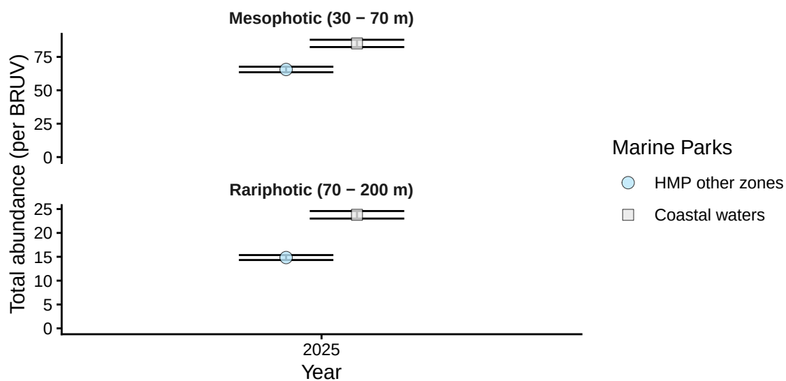
Figure A.8.1: Demersal fish - Total abundance: benchmark plots by zone and depth contour from stereo-BRUV groundtruthing. HMP = Hunter Marine Park (Commonwealth).
